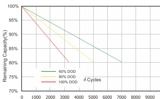
Different Discharge Depth Life Curves & 40°C, 0.5C
