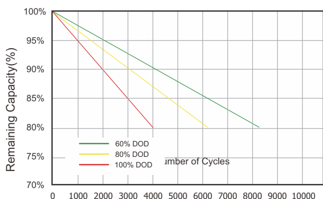
Different Discharge Depth Life Curves & 25°C, 0.5C
